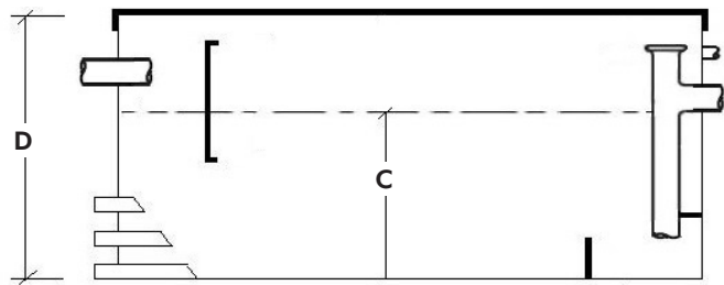
Section View
